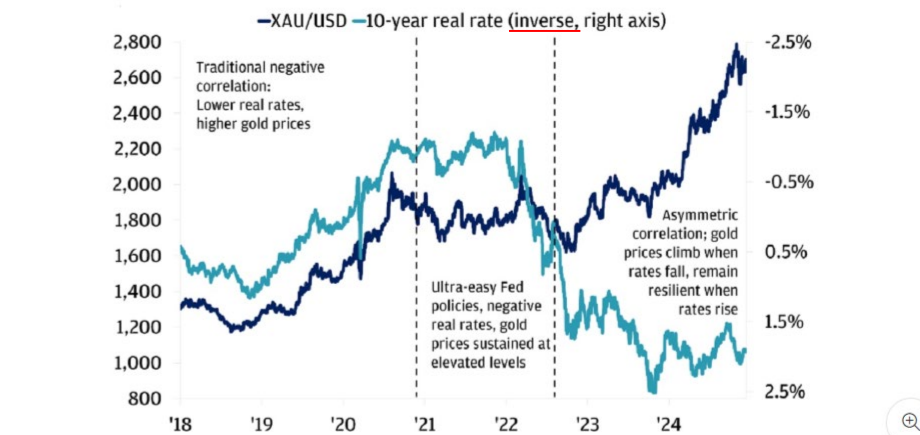
Gold prices vs 10-year U.S. real rate
